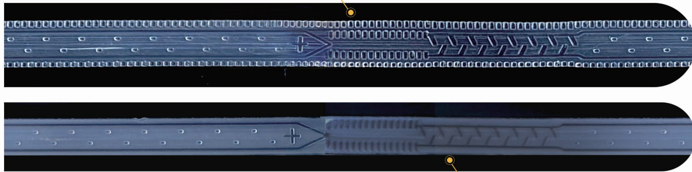
Traditional labyrinth drip tape
